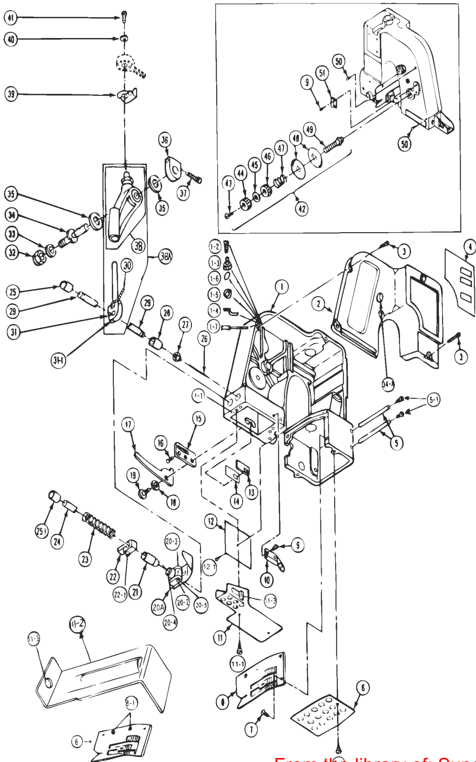
F302A MOD. "F300A" HOUSING, NEEDLE LEVER, PRESSER FOOT PLATE A ILLUSTRATED PARTS BREAKDOWN ORDER BY NUMBER
